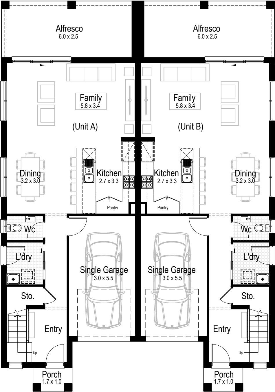
Ground Floor
