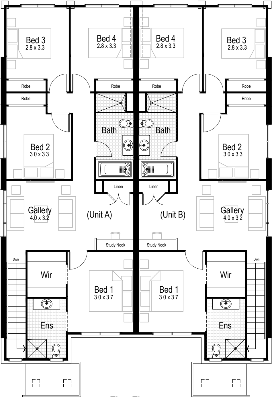
First Floor
