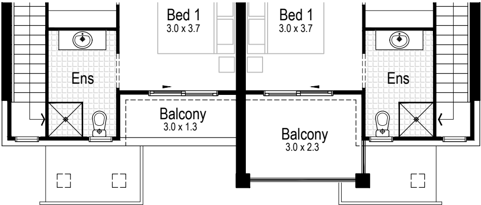
First Floor - Balcony Option
